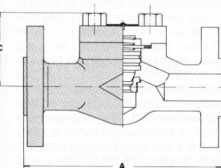
B-3674XU-F LIFT CHECK
