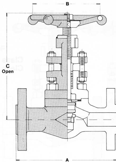
B-3644XU-F Integral Flanges
